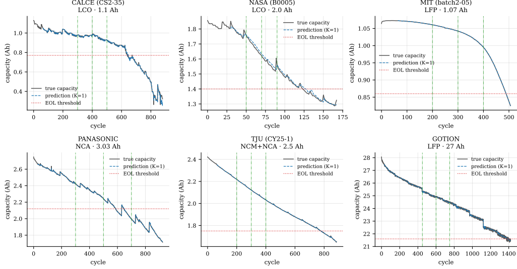
Figure 5: Single-step capacity prediction on one test cell per dataset. Green dashed lines mark the starting points (SPs); red dotted lines mark the EOL thresholds.
